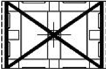
Figure H-11: Plan view Top 2 layers of pallet slats removed to show sling
