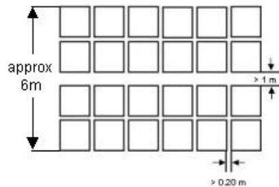
Figure F-2: Double row stack
