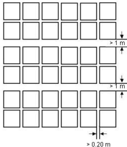
Figure F-3: In depth-stack
