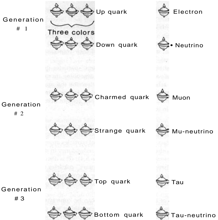
Figure 5.4. In the Standard Model, the first generation of particles consists of the "up" and "down" quark (in three colors, with their associated antiparticles) and the electron and neutrino. The embarrassing feature of the Standard Model is that there are three generation of such particles, each generation being nearly an exact copy of the previous generation. It's hard to believe that nature would be so redundant as to create, at a fundamental level, three identical copies of particles.
