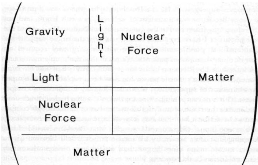
Figure 6.4. In supergravity, we almost get a unification of all the known forces (marble) with matter (wood). Like a jigsaw puzzle, they fit inside Riemann's metric tensor. This almost fulfills Einstein's dream.
