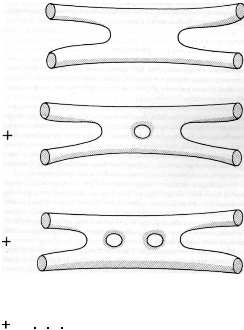
Figure 7.1. In string theory, the gravitational force is represented by the exchange of closed strings, which sweep out tubes in space-time. Even if we add up an infinite series of diagrams with a large number of holes, infinities never appear in the theory, giving us a finite theory of quantum gravity.
