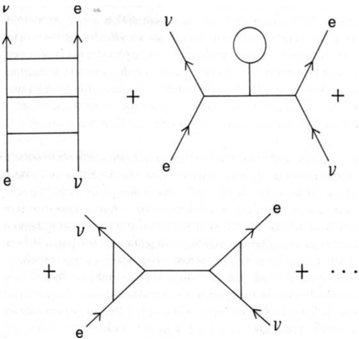
Figure 5.2. (a) In quantum theory, when subatomic particles bump into one another, they exchange packets of energy, or quanta. Electrons and neutrinos interact by exchanging a quantum of the weak force, called the W particle, (b) To calculate the complete interaction of electrons and neutrinos, we must add up an infinite series of graphs, called Feynman diagrams, where the quanta are exchanged in increasingly complicated geometric patterns. This process of adding up an infinite series of Feynman graphs is called perturbation theory.
