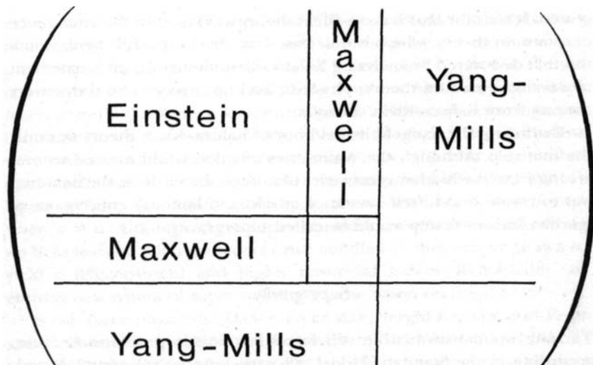
Figure 6.2. If we go to the N th dimension, then the metric tensor is a series of N^2 numbers that can be arranged in an N \times N block. By slicing off the fifth and higher columns and rows, we can extract the Maxwell electromagnetic field and the Yang-Mills field. Thus, in one stroke, the hyperspace theory allows us to unify the Einstein field (describing gravity), the Maxwell field (describing the electromagnetic force), and the Yang-Mills field (describing the weak and strong force). The fundamental forces fit together exactly like a jigsaw puzzle.
