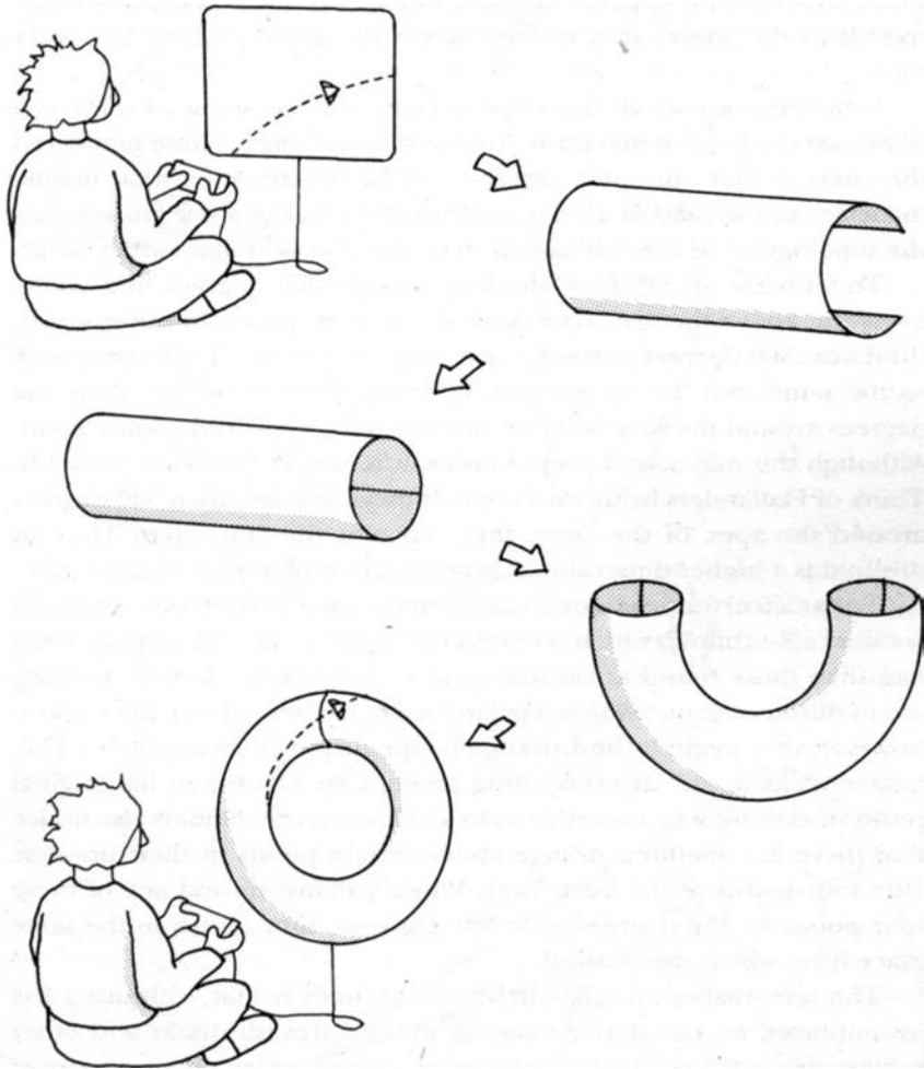
Figure 9.2. If a rocket disappears off the right side of a video-game screen, it re-emerges on the left. If it disappears at the top, it re-emerges at the bottom. Let us now wrap the screen so that identical points match. We first match the top and bottom points by wrapping up the screen. Then we match the points on the left- and right-hand sides by rolling up the screen like a tube. In this way, we can show that a video-game screen has the topology of a doughnut.
