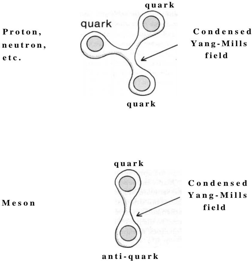
Figure 5.3. Strongly interacting particles are actually composites of even smaller particles, called quarks, which are bound together by a taffylike "glue," which is described by the Yang-Mills field. The proton and neutron are each made up of three quarks, while mesons are made up of a quark and an antiquark.
