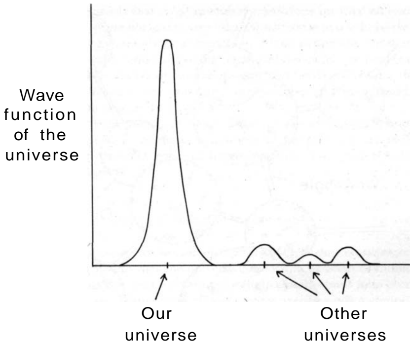
Figure 12.1. In Hawking's wave function of the universe, the wave function is most likely concentrated around our universe. We live in our universe because it is the most likely, with the largest probability. However, there is a small but non-vanishing probability that the wave function prefers neighboring, parallel universes. Thus transitions between universes may be possible (although with very low probability).
