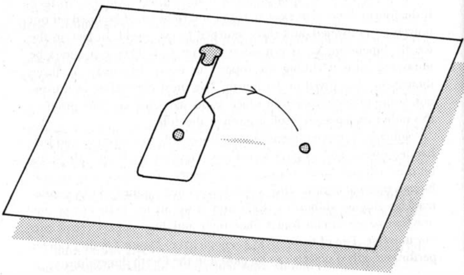
Figure 2.8. The mystic Henry Slade claimed to be able to change right-handed snail shells into left-handed ones, and to remove objects from sealed bottles. These feats are impossible in three dimensions, but are trivial if one can move objects through the fourth dimension.
