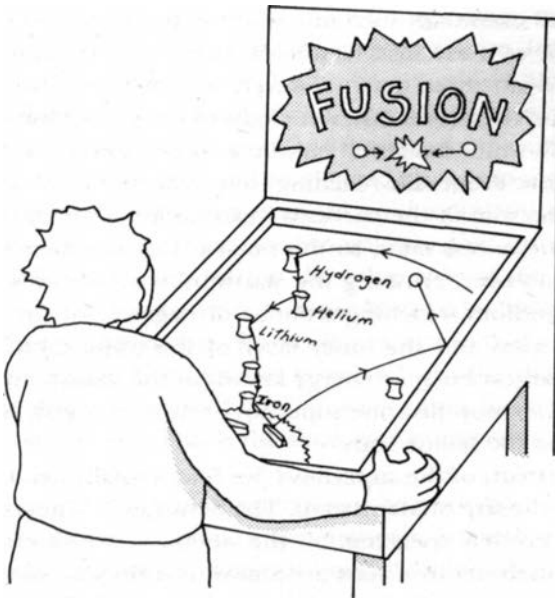
Figure 10.1. The average "weight" of each proton of lighter elements, such as hydrogen and helium, is relatively large. Thus if we fuse hydrogen to form helium inside a star, we have excess mass, which is converted to energy via Einstein's equation E = mc^2 . This is the energy that lights up the stars. But as stars fuse heavier and heavier elements, eventually we reach iron, and we cannot extract any more energy. The star then collapses, and the tremendous heat of collapse creates a supernova. This colossal explosion rips the star apart and seeds the interstellar space, in which new stars are formed. The process then starts all over again, like a pinball machine.
