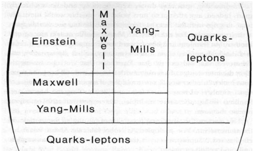
Figure 6.3. Supergravity almost fulfills Einstein's dream of giving a purely geometric derivation of all the forces and particles in the universe. To see this, notice that if we add supersymmetry to the Riemann metric tensor, the metric doubles in size, giving us the super Riemann metric. The new components of the super Riemann tensor correspond to quarks and leptons. By slicing the super Riemann tensor into its components, we find that it includes almost all the fundamental particles and forces in nature: Einstein's theory of gravity, the Yang-Mills and Maxwell fields, and the quarks and leptons. But the fact that certain particles are missing in this picture forces us to go a more powerful formalism: superstring
