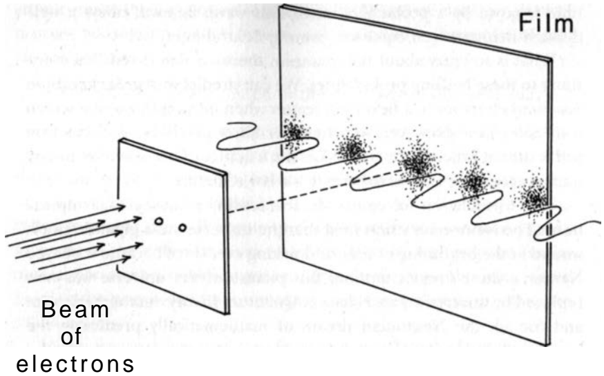
Figure 5.1. A beam of electrons is shot through two small holes and exposes some film. We expect to see two dots on the film. Instead, we find an undulating interference pattern. How can this be? According to quantum theory, the electron is indeed a pointlike particle and cannot go through both holes, but the Schrodinger wave associated with each electron can pass through both holes and interfere with itself.
